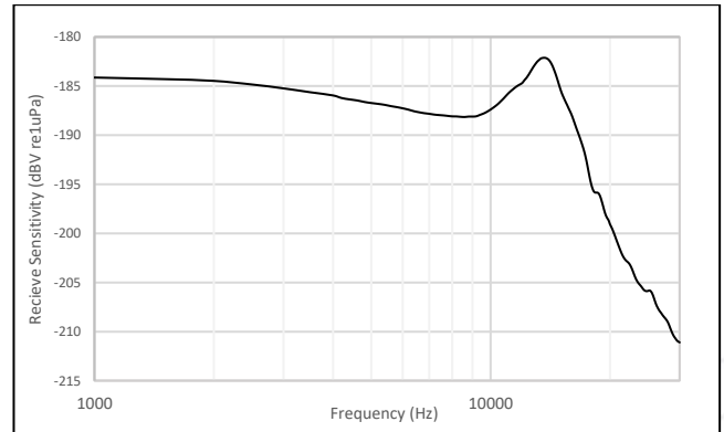
Figure 2: Receive Sensitivity Plot for M18C-6.0
