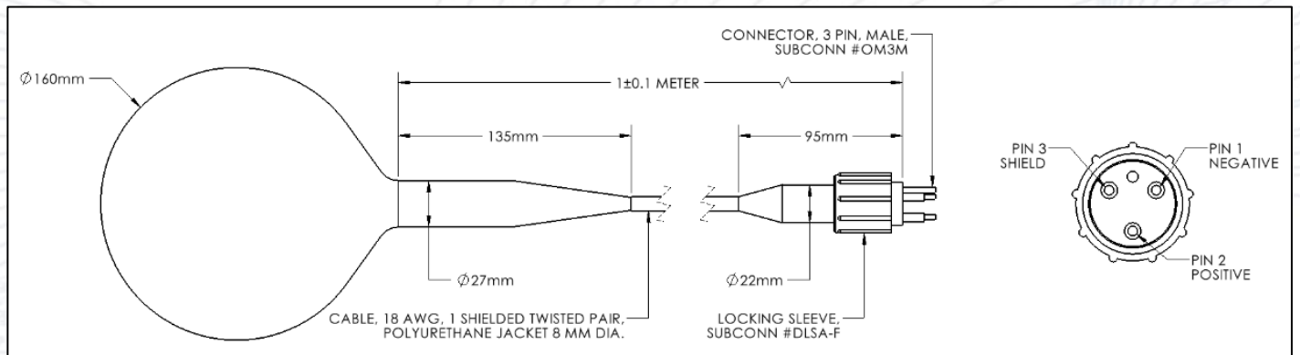
Figure 4: Dimensions of the M18C-6.0 Sphere with labeled pinout
