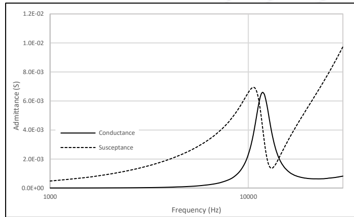
Figure 3: Admittance Plot for M18C-6.0
