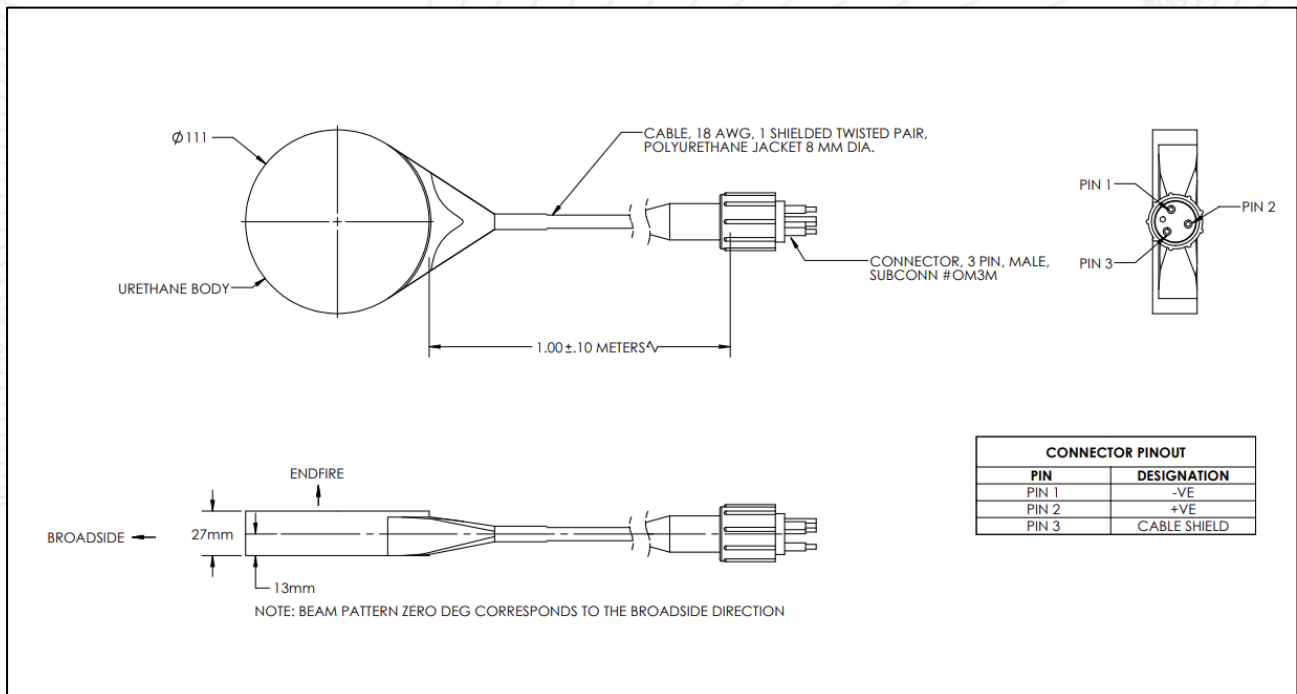
Figure 5: Dimensions of the M21-100-2000 with labeled pin out
