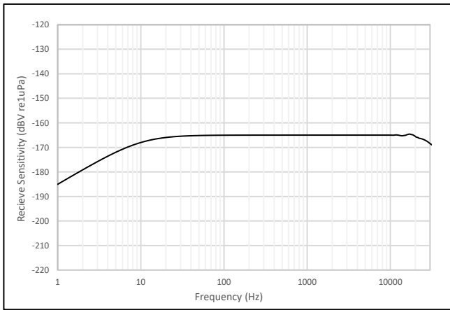
Figure 1: Nominal Receive Sensitivity Plot for M36-014 (With Standard Pre-Amp)
