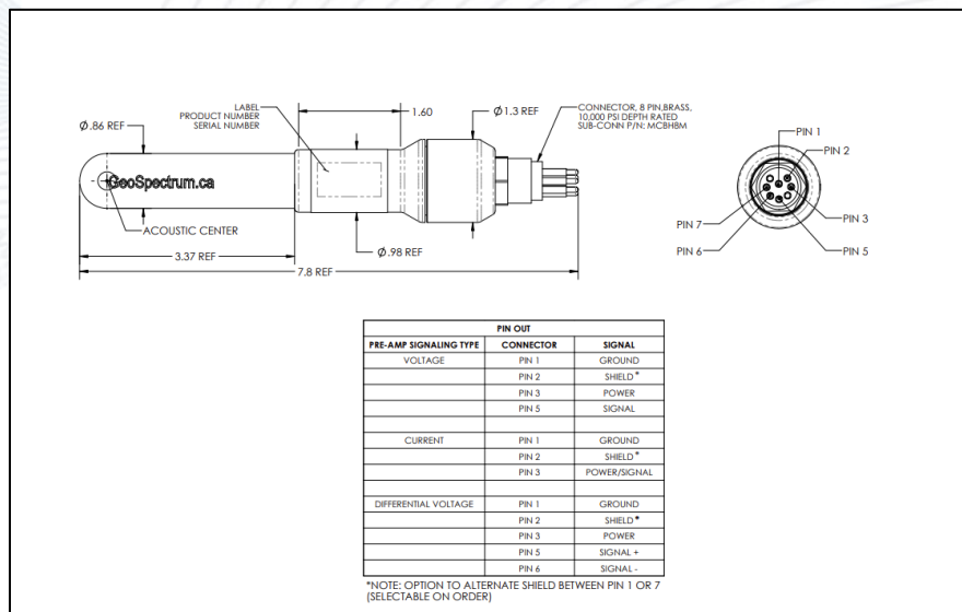
Figure 5: Dimensions of the M36-014 Hydrophone with labeled pin out
