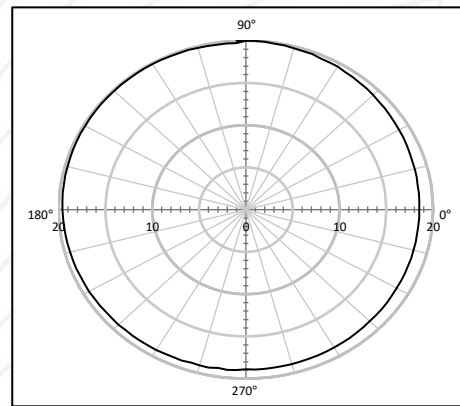
Figure 4: Typical Horizontal Beam Pattern for the M36-014 @ 30 kHz
