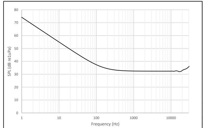
Figure 2: SPL Equivalent Self Noise Plot for M36-014
