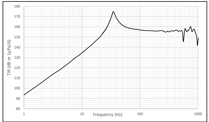
Figure 2: Transmit Current Response for M72-30
