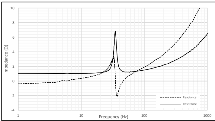
Figure 3: Impedance Plot for M72-30
