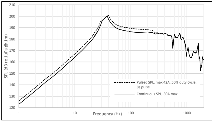
Figure 1: Sound Pressure Level Limits Plot for M72-30 with M620-210 Amplifier Limit and Cable Impedance of 1Ω
