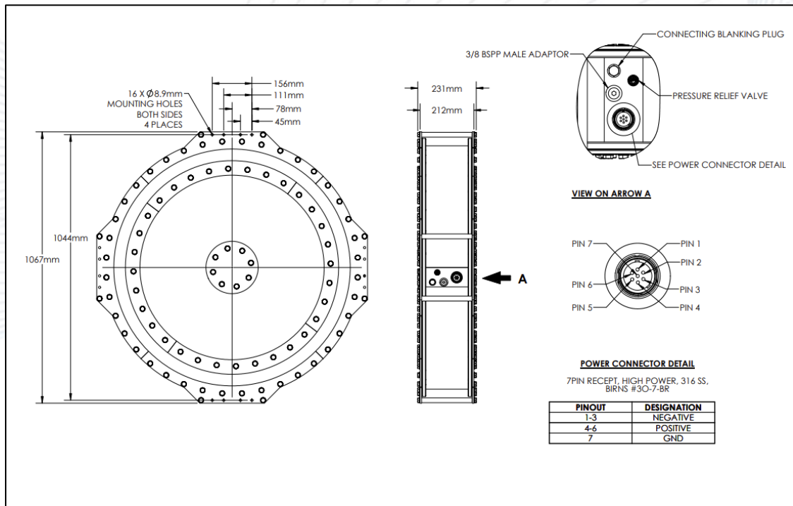
Figure 5: Dimensions of the M72-30 with labeled pin out
