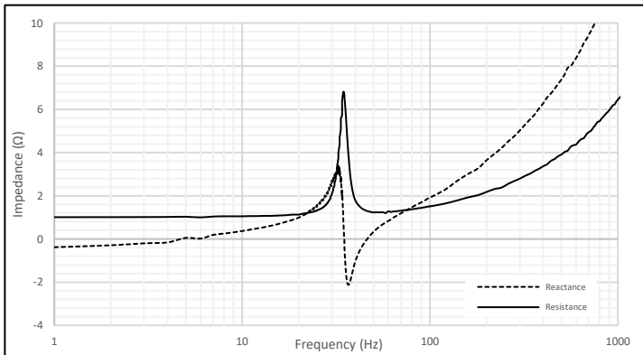
Figure 3: Impedance Plot for M72-30
