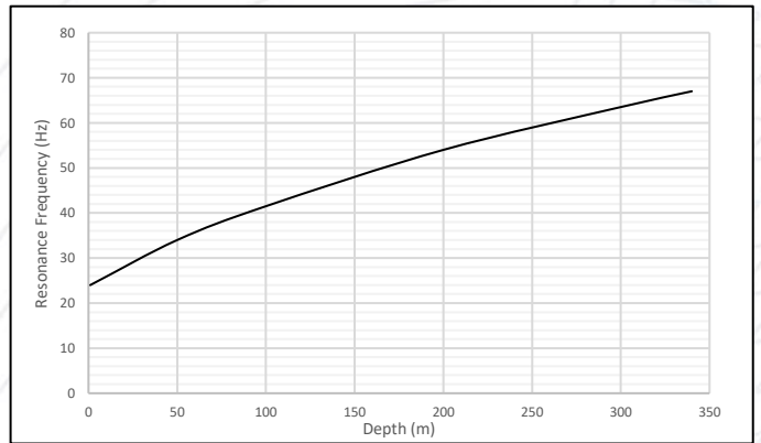
Figure 4: Modelled Resonance Frequency vs Depth
