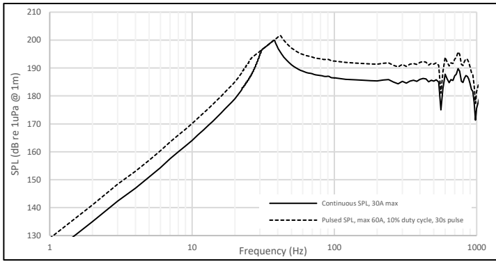
Figure 1: Sound Pressure Level Limits Plot for M72-30
