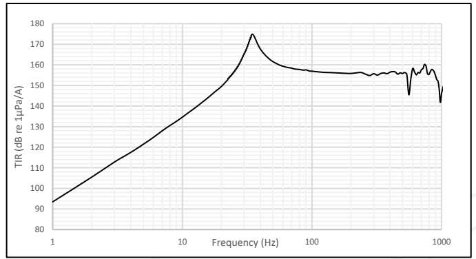
Figure 2: Transmit Current Response for M72-30
