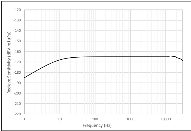
Figure 1: Nominal Receive Sensitivity Plot for M36-014 (With Standard Pre-Amp)
