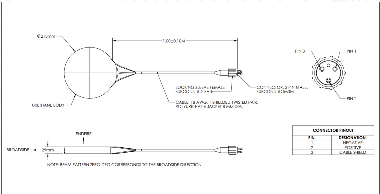
Figure 5: Dimensions of the M21-203-500 with labeled pin out
