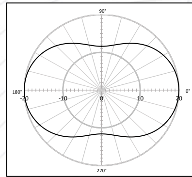
Figure 4: Typical Horizontal Beam Pattern for the M21-203-500 at 2000Hz
