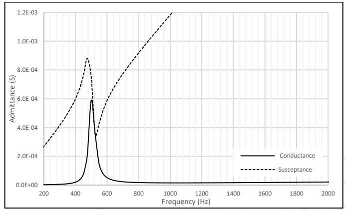
Figure 2: Admittance Plot for M21-203-500
