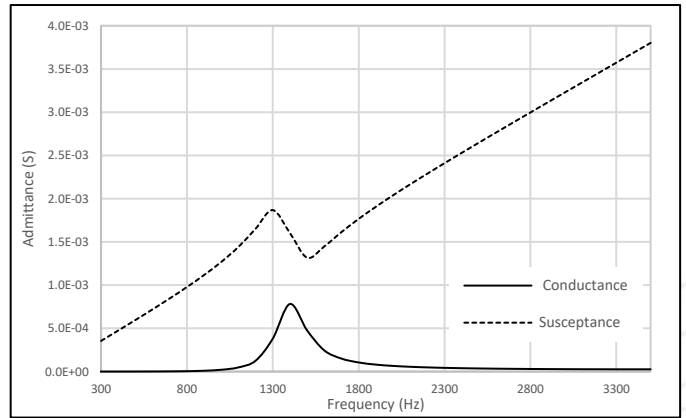
Figure 2: Admittance Plot for M21-203-1400
