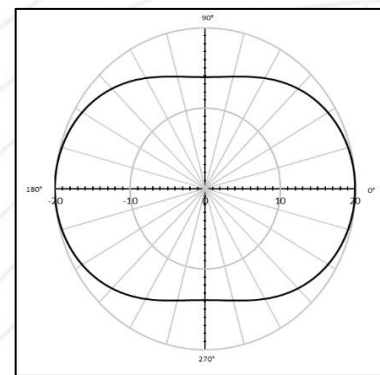
Figure 4: Typical Horizontal Beam Pattern for the M21-203-1400 at 3500Hz
