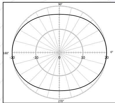
Figure 4: Typical Vertical Beam Pattern for the M21-100-3000 at 4500Hz
