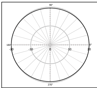
Figure 3: Typical Horizontal Beam Pattern for the M21-100-3000 at Resonance Frequency
