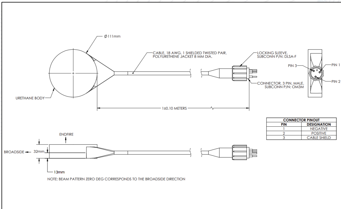
Figure 5: Dimensions of the M21-100-3000 with labeled pin out
