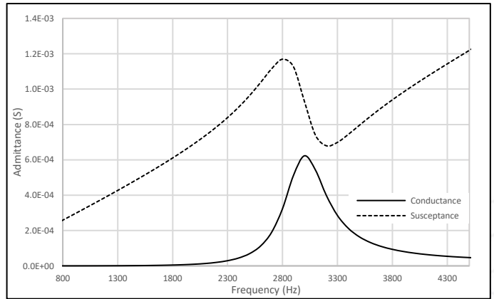
Figure 2: Admittance Plot for M21-100-3000
