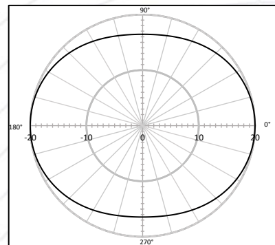
Figure 4: Typical Horizontal Beam Pattern for the M21-100-3000 at 4500Hz
