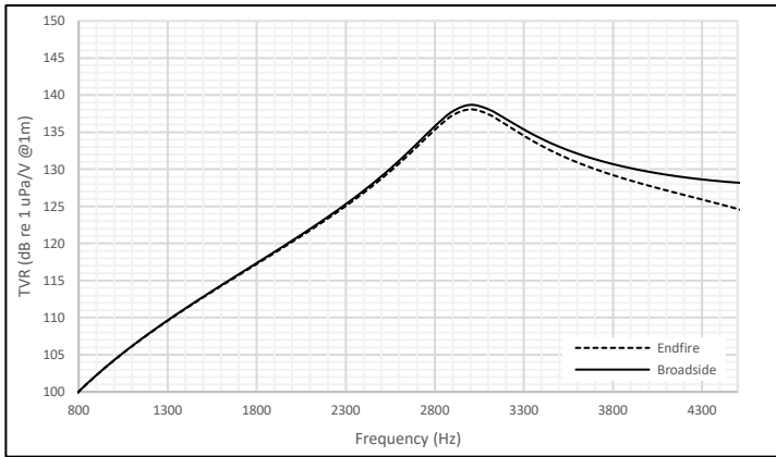
Figure 1: Transmit Voltage Response for M21-100-3000
