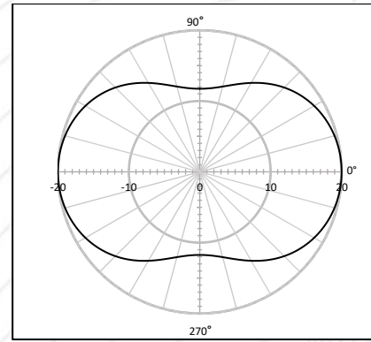
Figure 4: Typical Vertical Beam Pattern for the M21-070-5000 at 10kHz
