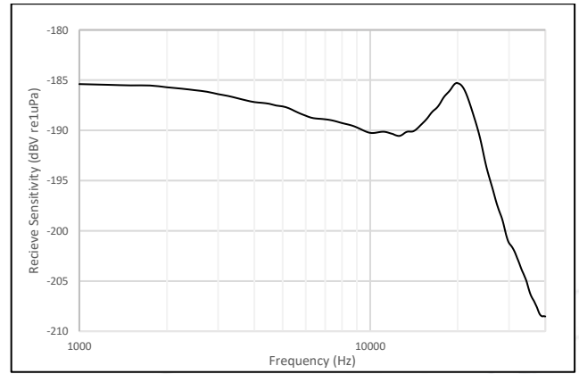
Figure 2: Receive Sensitivity Plot for M18C-4.0
