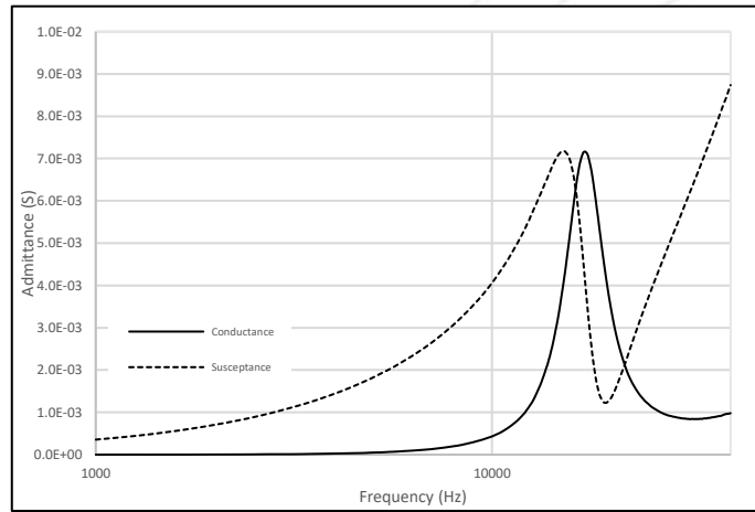
Figure 3: Admittance Plot for M18C-4.0
