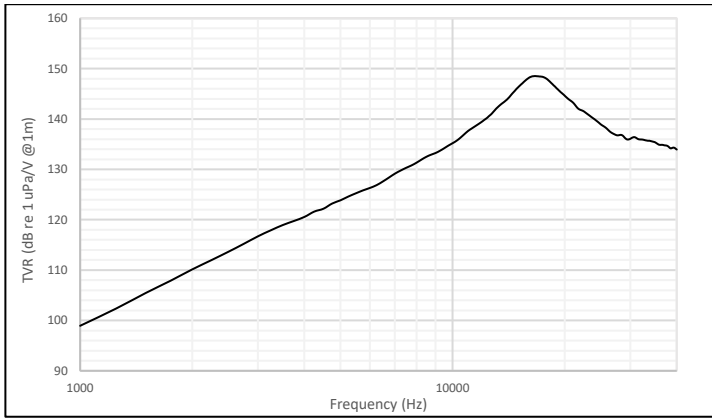
Figure 1: Transmit Voltage Response for M18C-4.0
