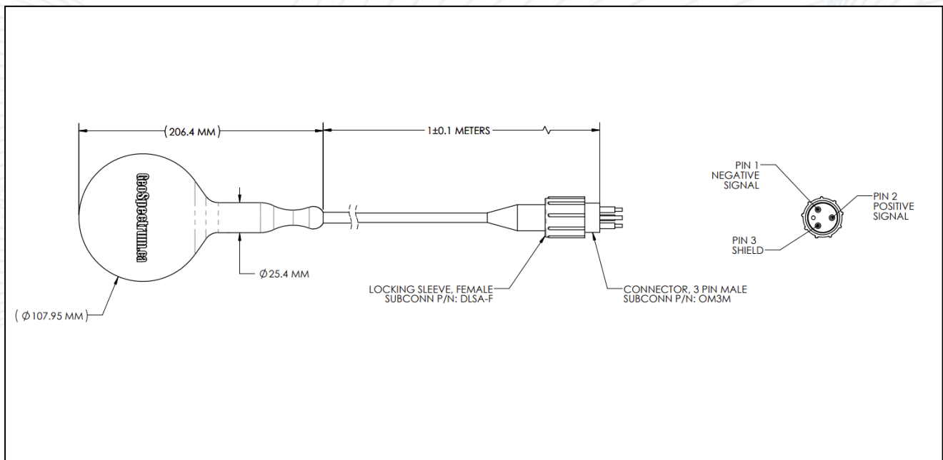
Figure 4: Dimensions of the M18C-4.0 with labeled pin out
