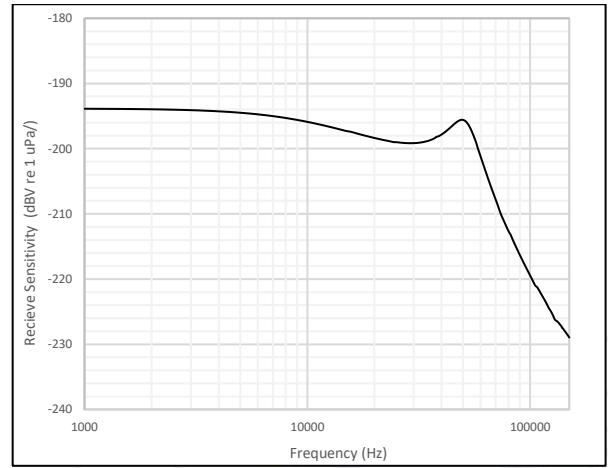
Figure 2: Receive Sensitivity Plot for M18C-1.5
