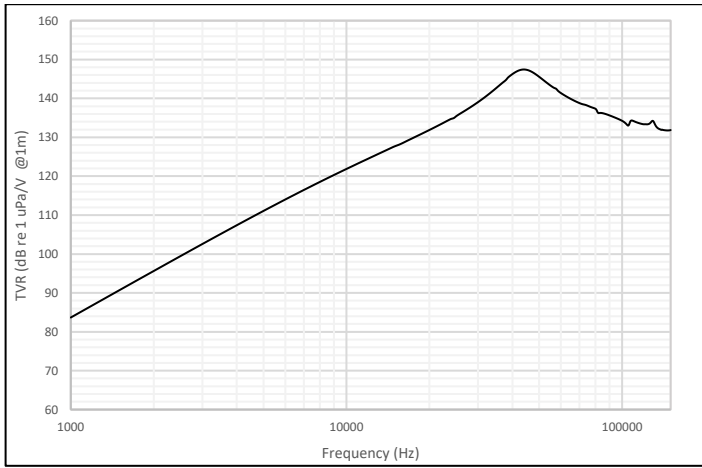
Figure 1: Transmit Voltage Response for M18C-1.5
