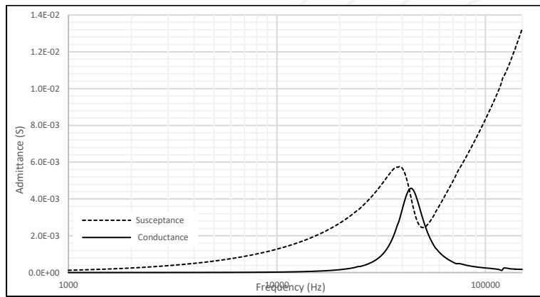
Figure 3: Admittance Plot for M18C-1.5
